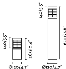
Post Lamp Ref. 70767
